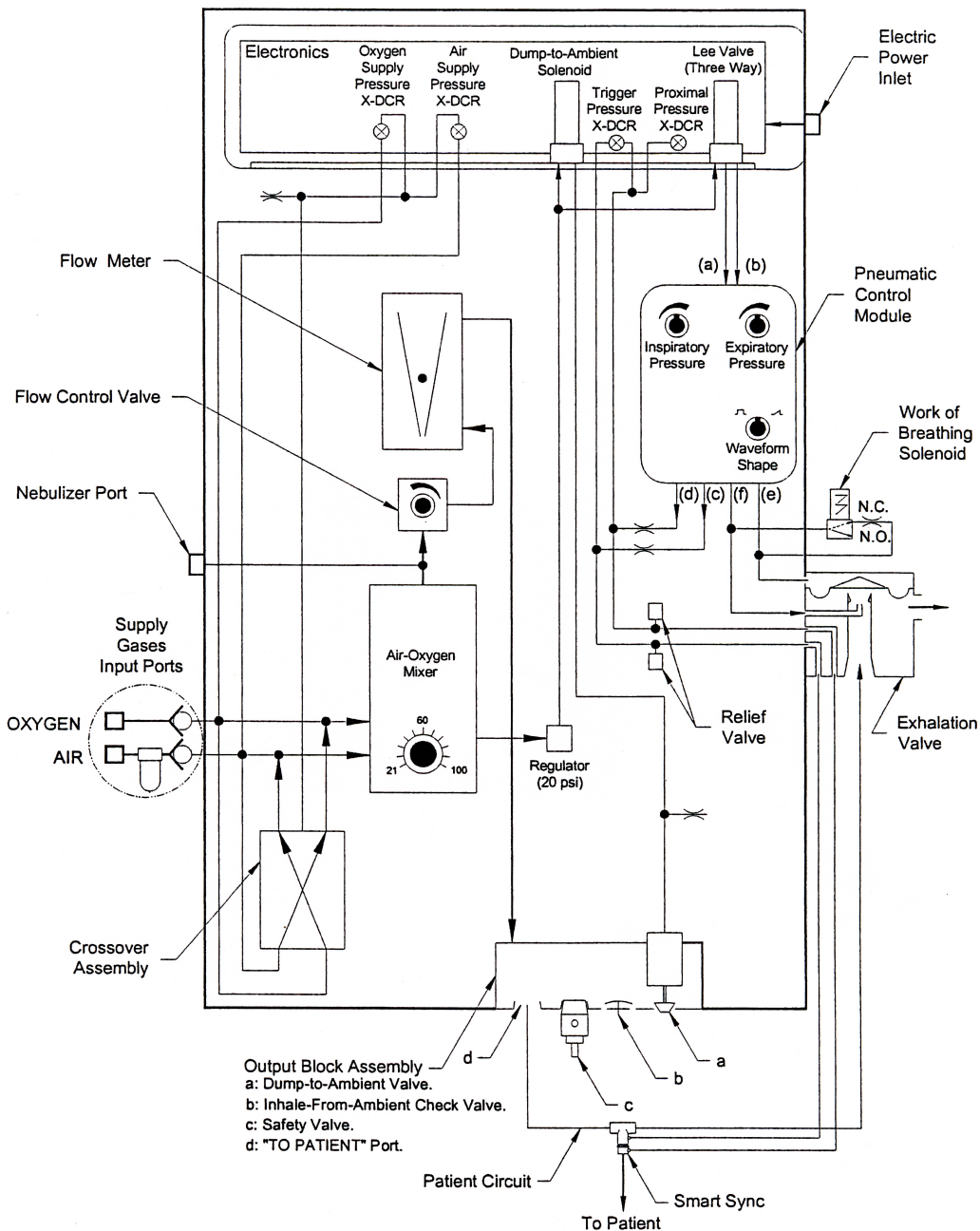
Schematic of Millennium® Ventilator's Pneumatic System
