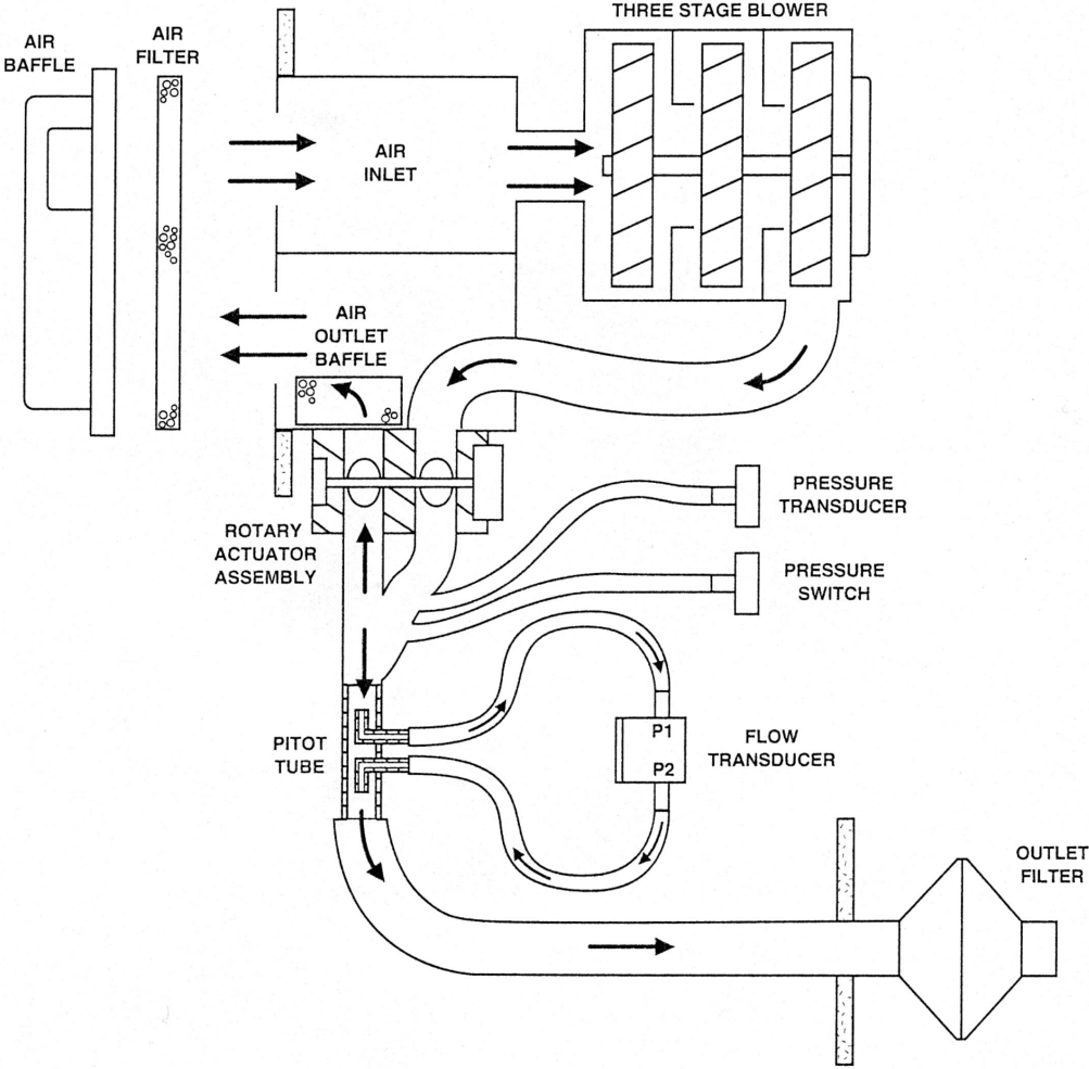
Pneumatic Diagram
